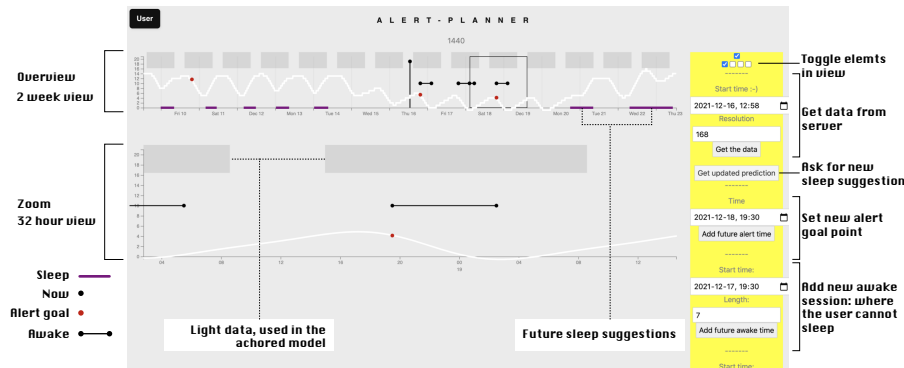
Figure 2: Awari with a stochastic brute-force sleep planner
